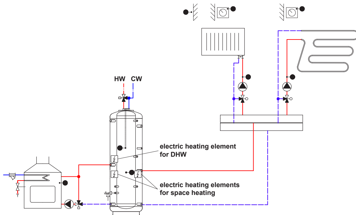
Hydraulic variant 1: Fireplace combined with electric heating elements
