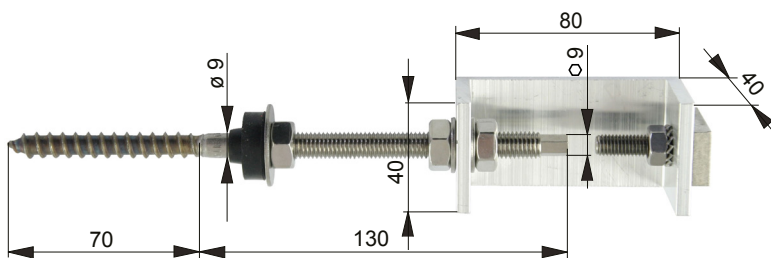
d) Hanger bolt for rail fixing
