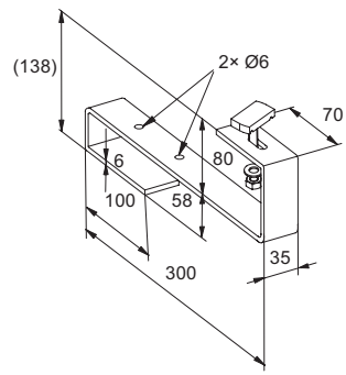
b) Roof anchor of stainless steel or zinc-plated steel for pantiles
