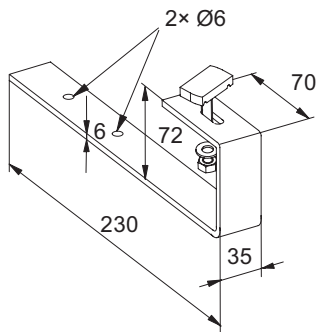
c) Stainless steel roof anchor for metal or slate roofing
